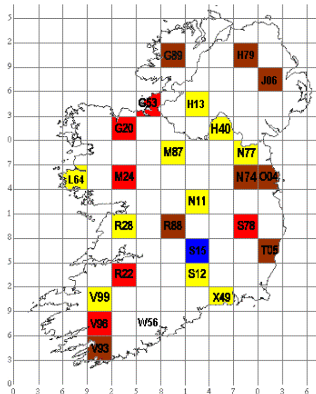
Figure 11: Survey blocks colour coded according to soprano pipistrelle encounter rates (per hour). Map shows average encounter data from both surveys 2006 where data for both surveys is available. The overall average rate of soprano pipistrelle encounters for 2006 was 9.75\text{hr}^{-1} . Squares are not highlighted if no data is available.
