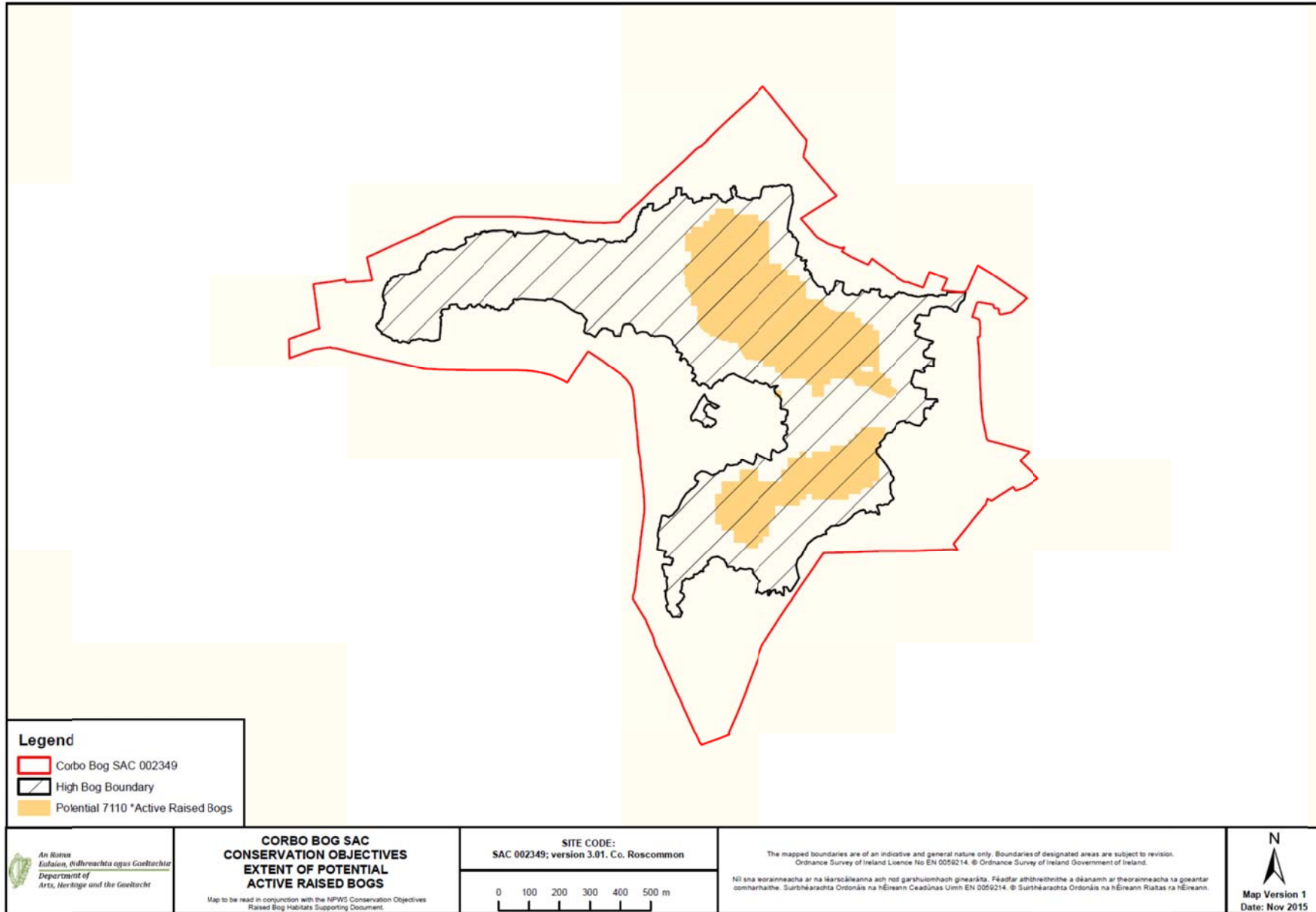
Map 1: Extent of potential active raised bog on Corbo Bog.
