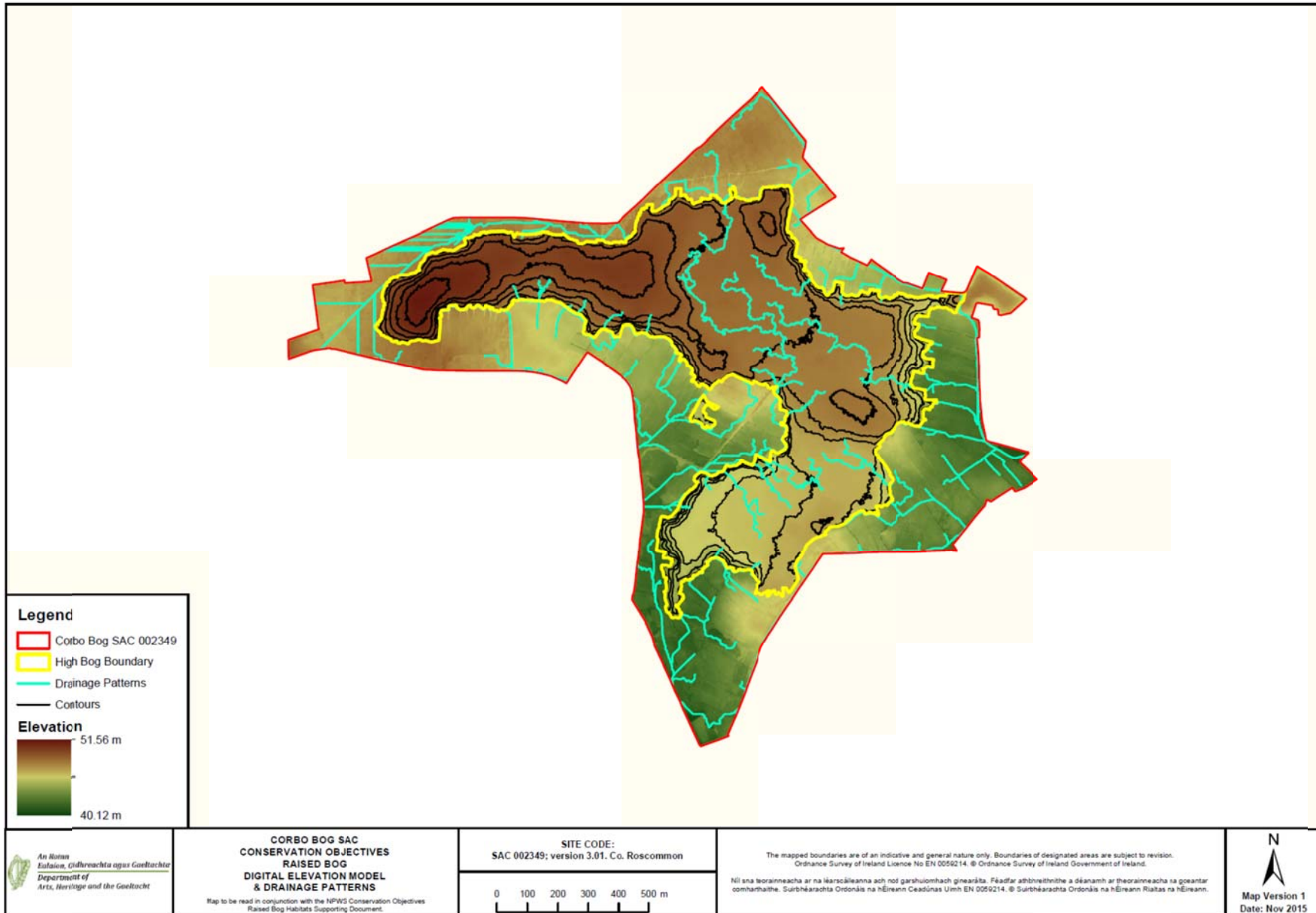
Map 3: Digital elevation model and drainage patterns at Corbo Bog.
