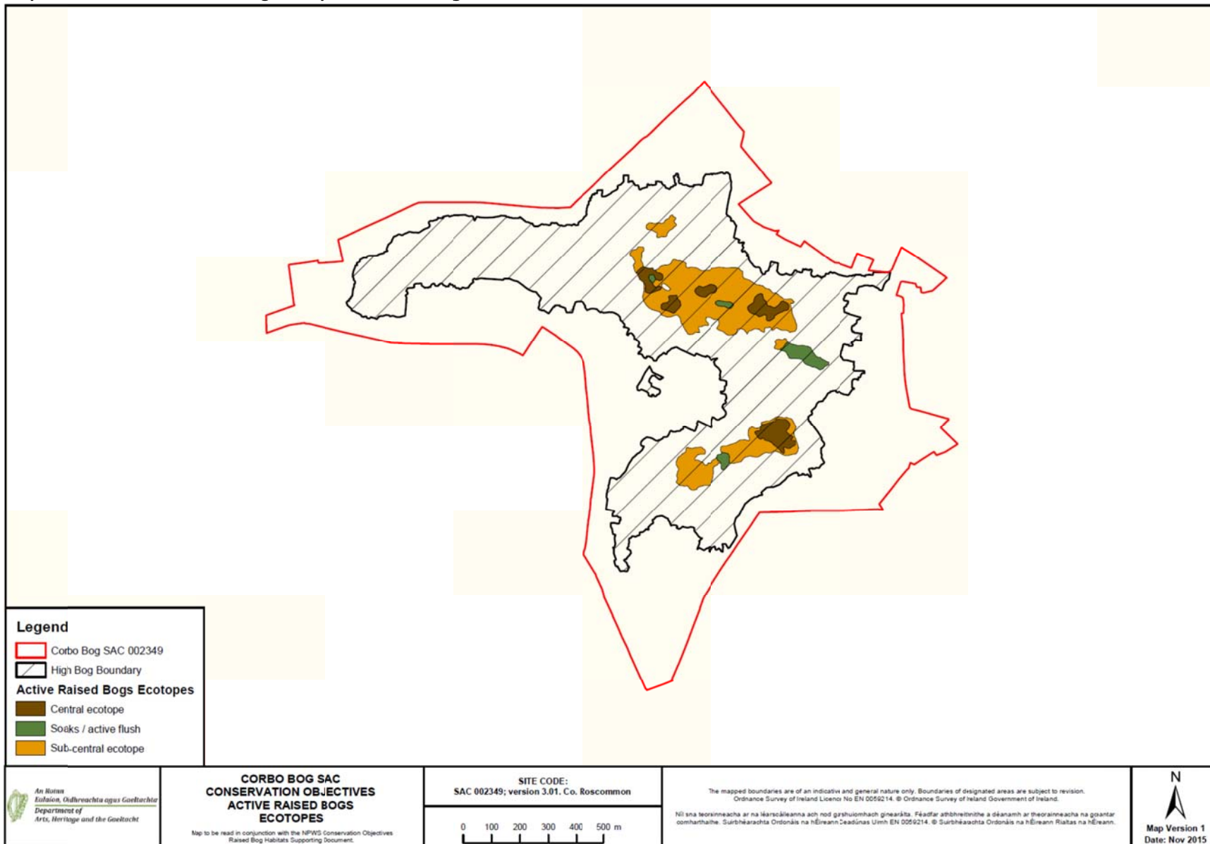
Map 2: Distribution of raised bog ecotopes on Corbo Bog.
