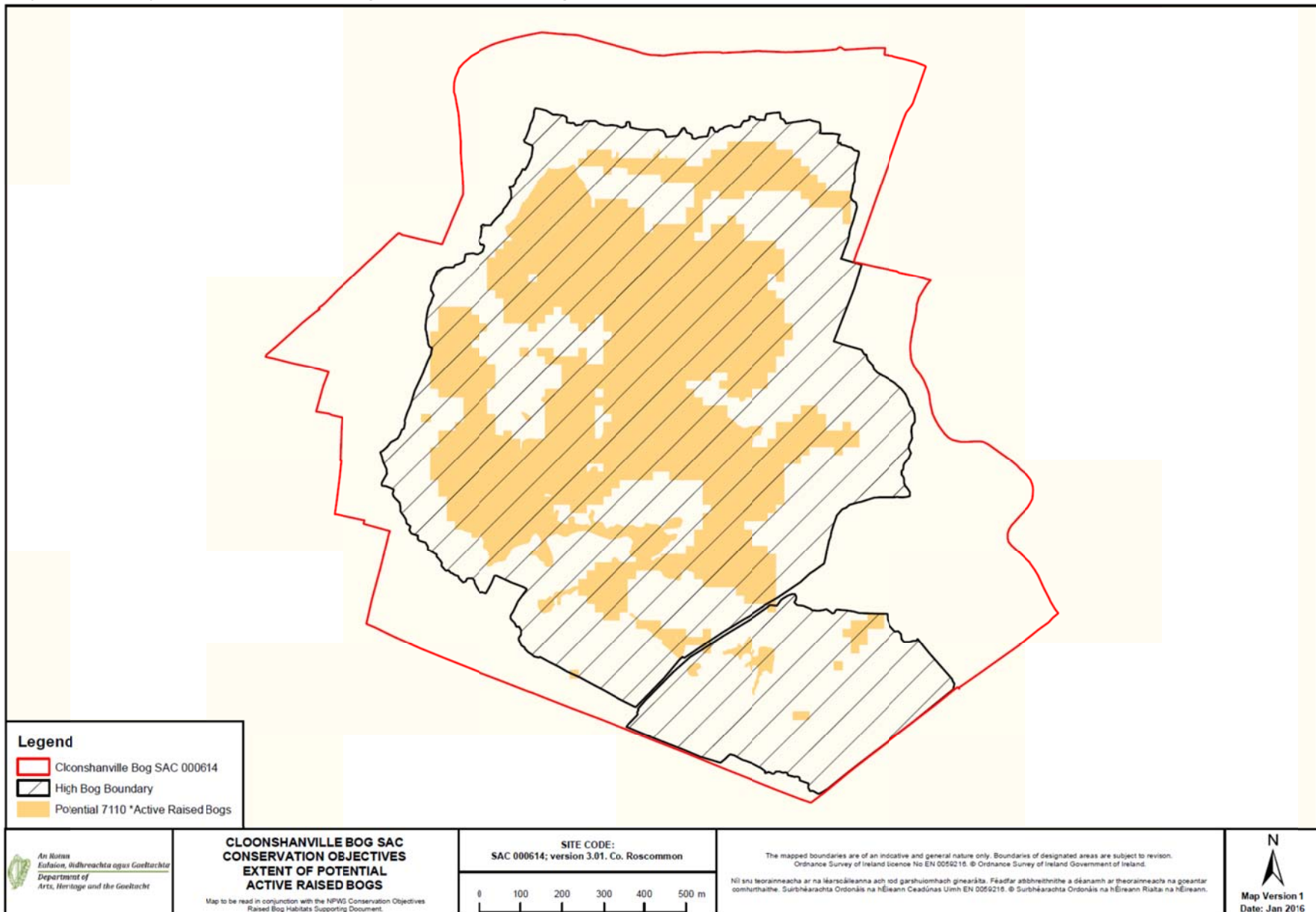
Map 1: Extent of potential active raised bog on Cloonshanville Bog.
