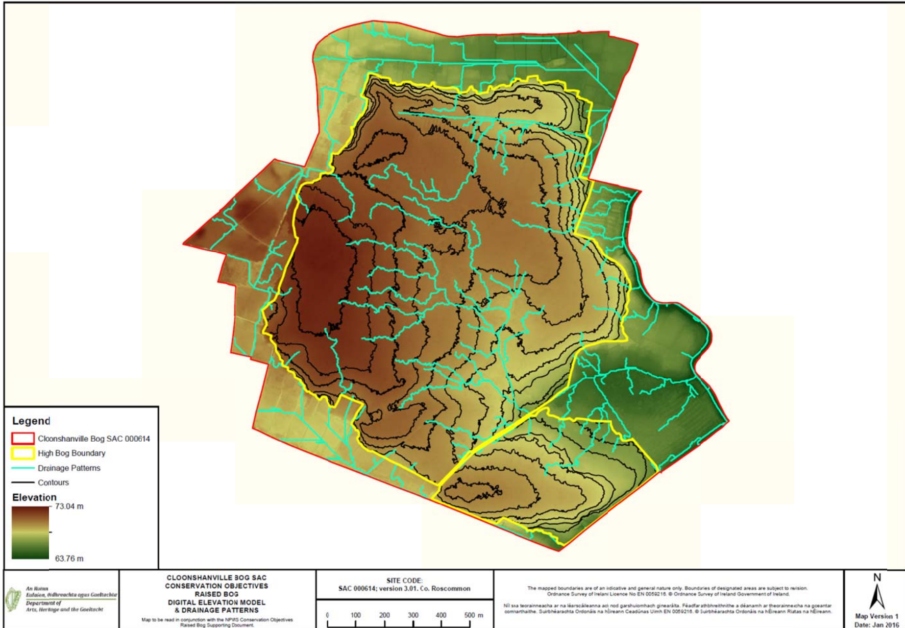
Map 3: Digital elevation model and drainage patterns at Cloonshanville Bog.
