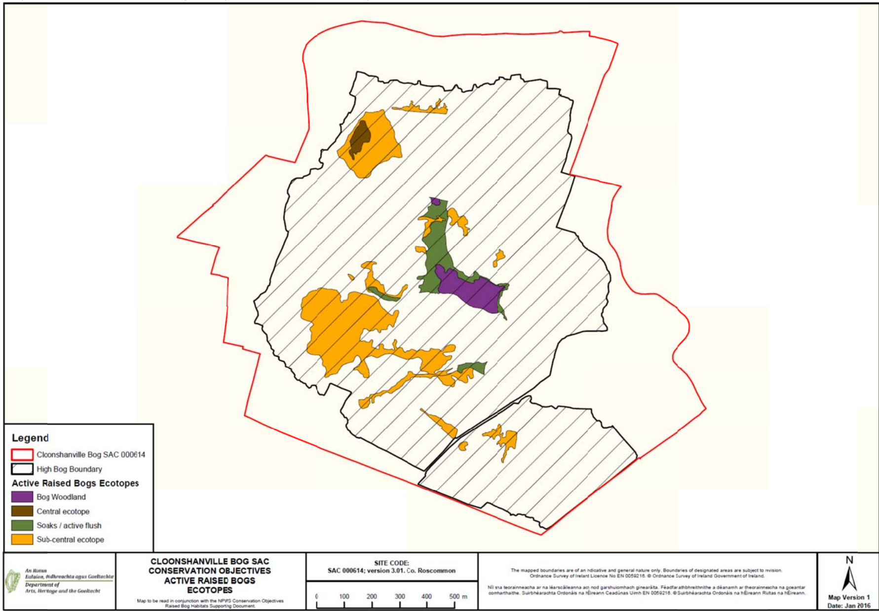
Map 2: Distribution of raised bog ecotopes on Cloonshanville Bog.
