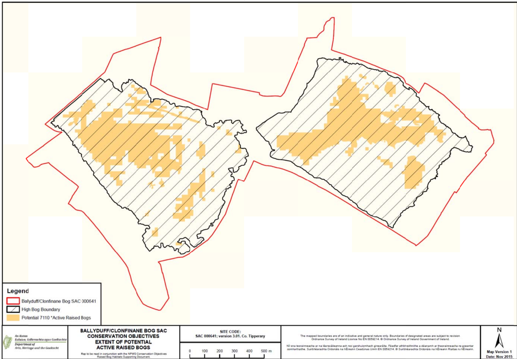
Map 1: Extent of potential active raised bog on Ballyduff/Clonfinane Bog.
