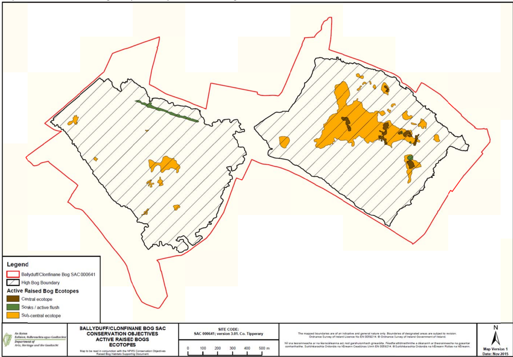
Map 2: Distribution of raised bog ecotopes on Ballyduff/Clonfinane Bog.
