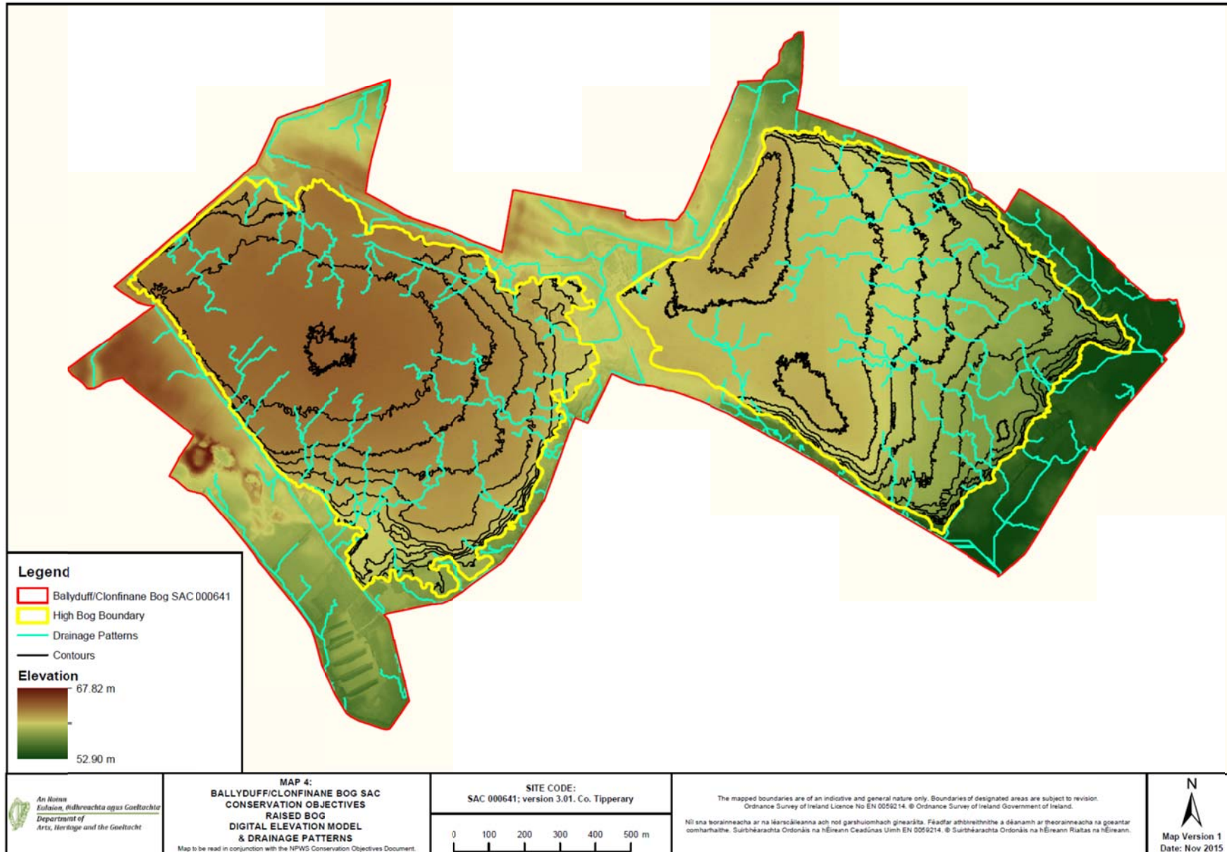
Map 3: Digital elevation model and drainage patterns at Ballyduff/Clonfinane Bog.
