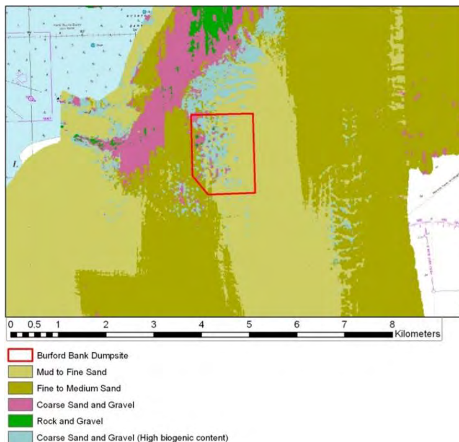
Figure 7-11 Sediment characterisation across the seabed of the dumpsite disposal area. Data reproduced from INFOMAR (2010)
