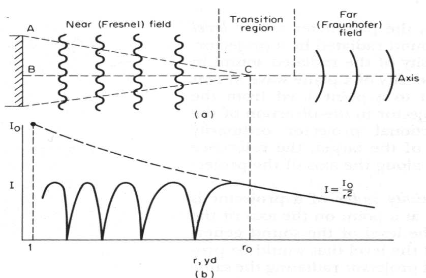
Figure 12-2 Underwater Noise source level fields (Urich 1983, fig. 4)
