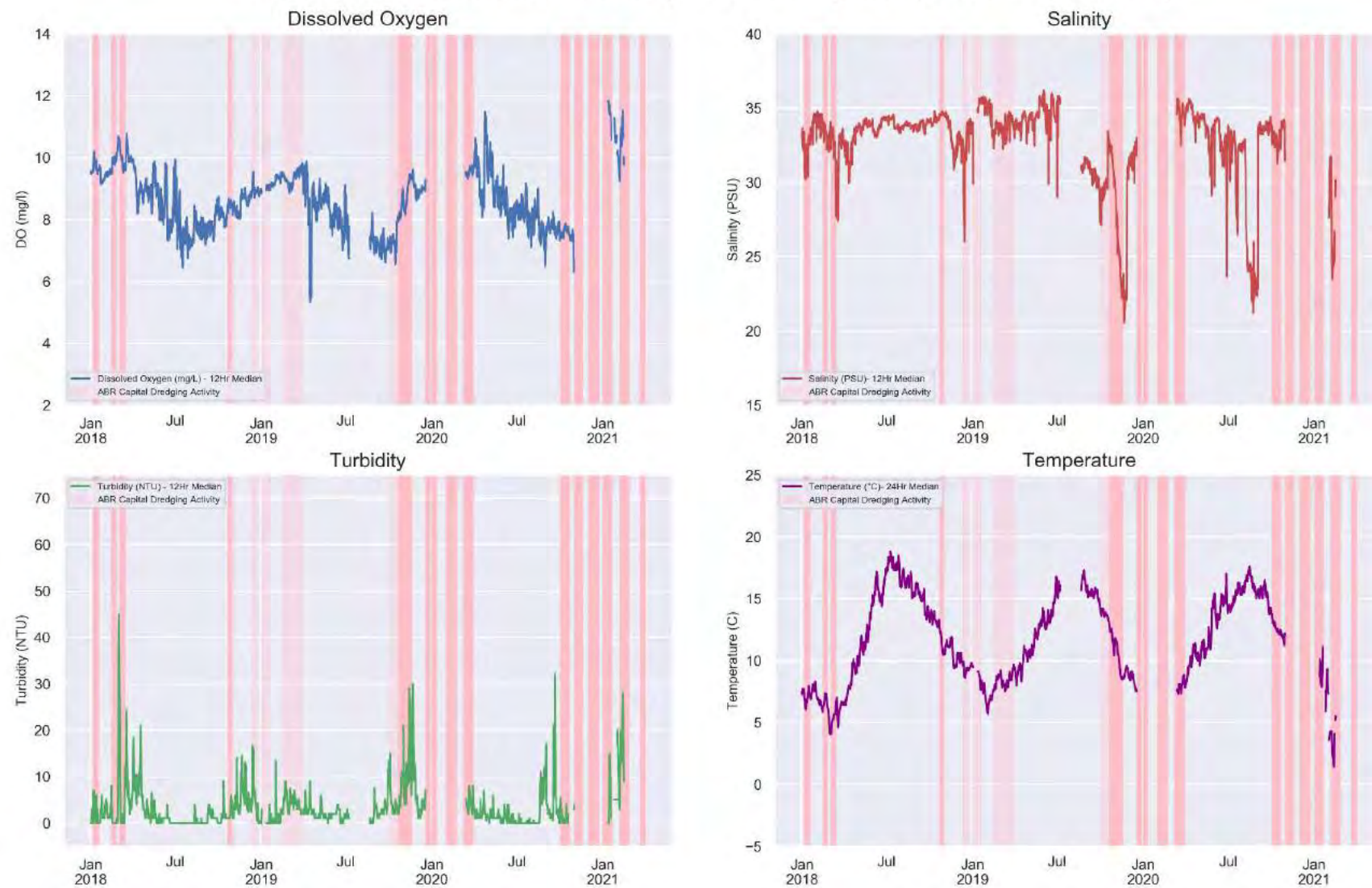
Figure 9-12 North Bank Monitoring Station - Water Quality Data (12 Hour Median)
