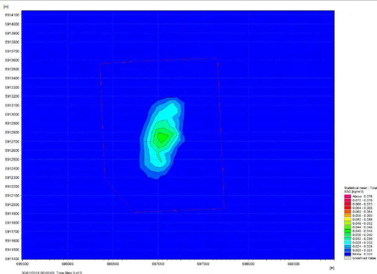
Figure 13-29 Mean Total Suspended Solids Concentration envelope using a Trailer Suction Dredger dumping hopper load of 4,100m 3 at 3 hourly intervals on average
