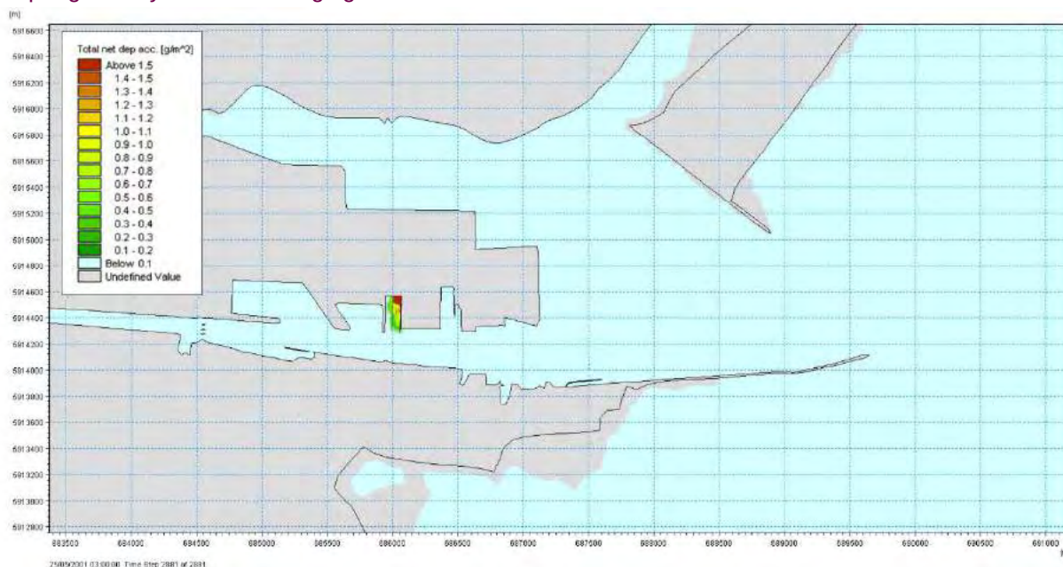
Figure 13-20 Deposition of sediment following the dredging operations within the Oil Berth
