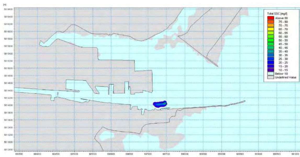
Figure 13-22 Suspended sediment concentration plume in the bottom layer during a typical mid flood phase of a spring tidal cycle during the capital dredging works
