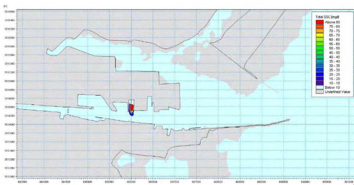
Figure 13-16 Suspended sediment concentration plume in the bottom layer during a typical low water phase of a spring tidal cycle whilst dredging within the Oil Berth
