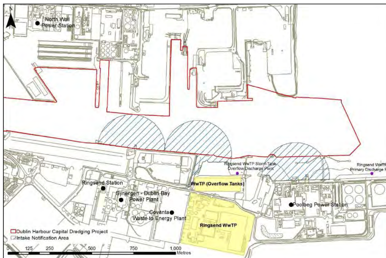
Figure 13-26 Locations of cooling water intakes in Dublin Harbour
