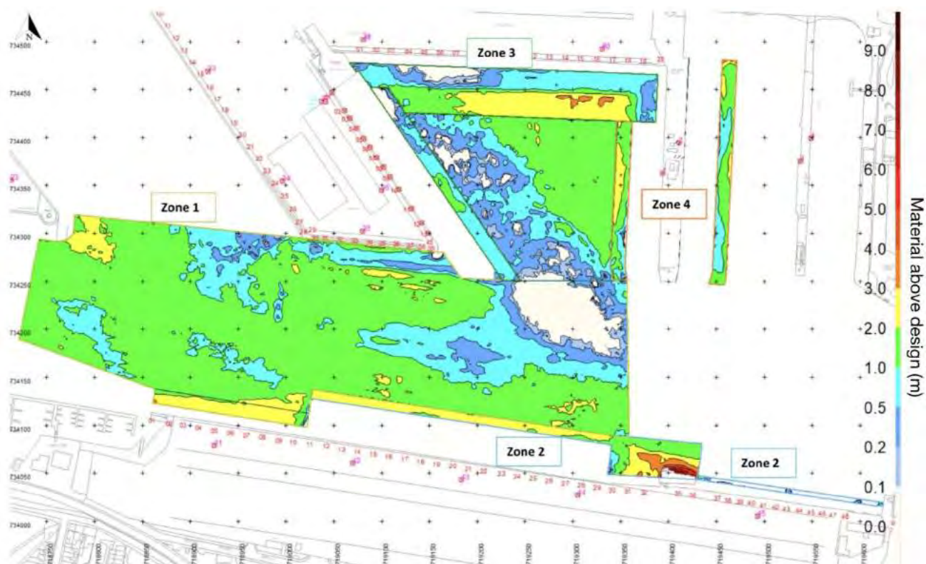
Figure 3-2 Plot showing depth of material between current bed level and design depth (metres) – Zone 1,2,3 and 4
