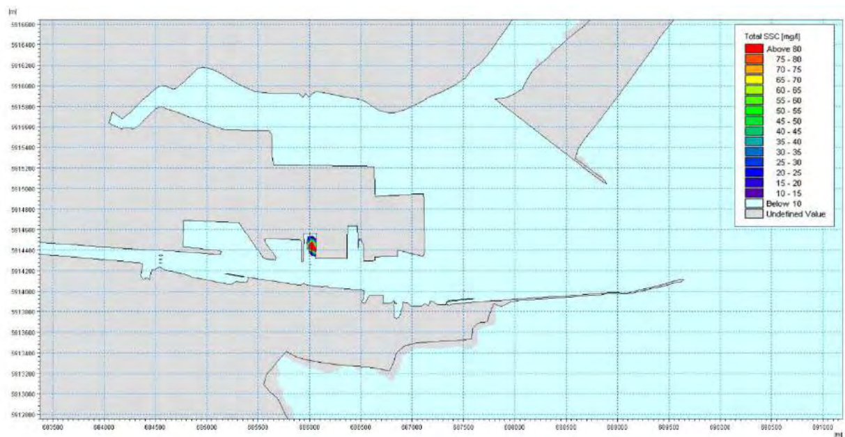
Figure 13-18 Suspended sediment concentration plume in the bottom layer during a typical high water phase of a spring tidal cycle whilst dredging within the Oil Berth
