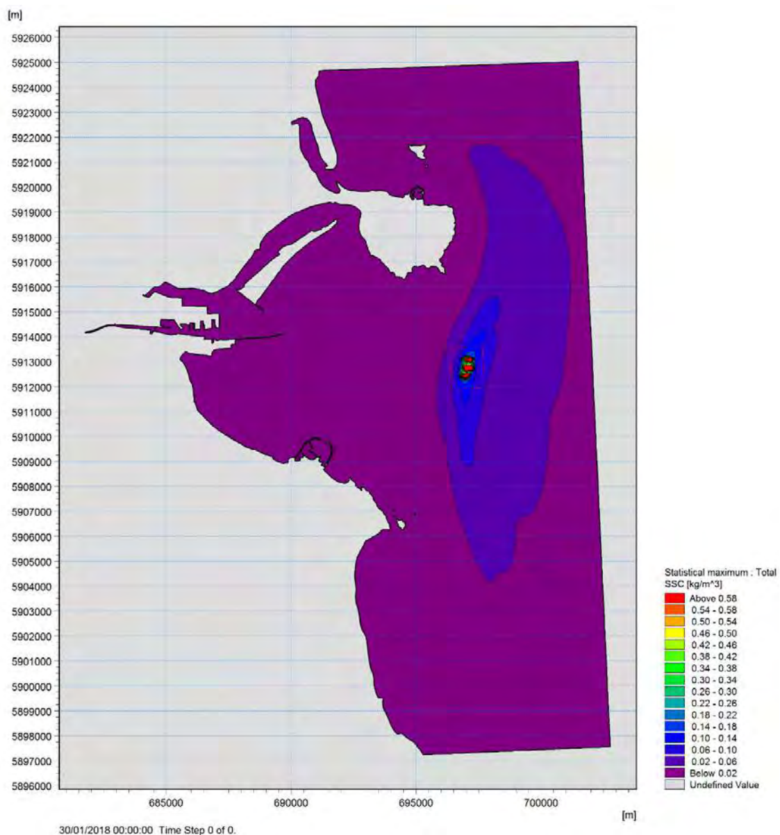
Figure 13-28 Maximum Total Suspended Solids Concentration envelope using a Trailer Suction Dredger dumping hopper load of 4,100m³ at 3 hourly intervals on average
