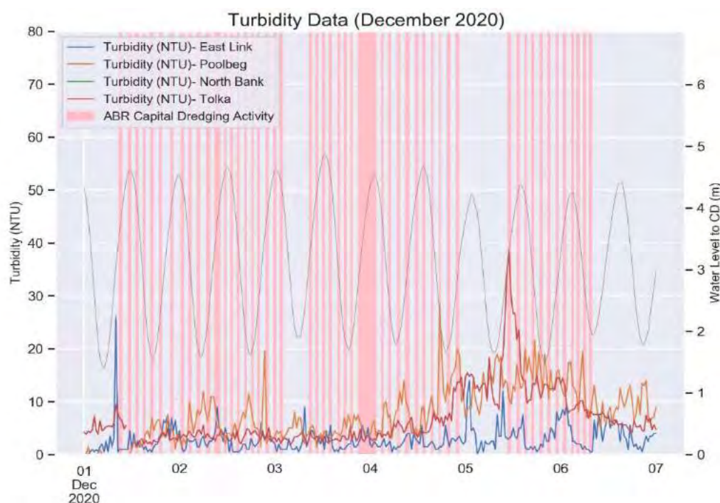
Figure 9-17 Turbidity and dredging activity from 1st December 2020 to 7th December 2020
