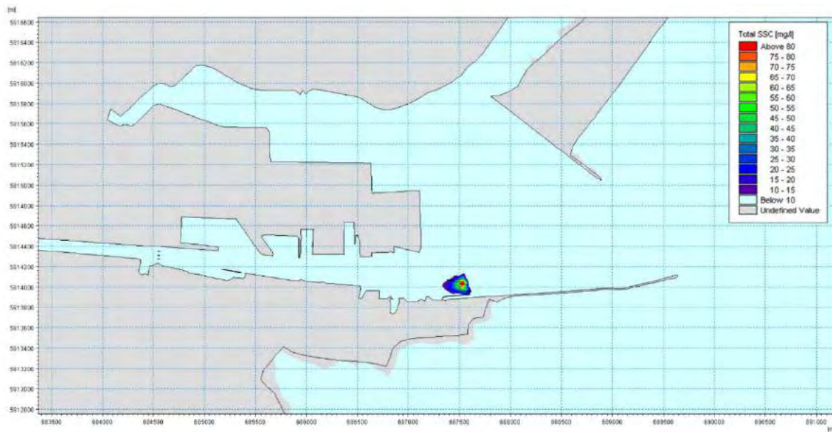
Figure 13-23 Suspended sediment concentration plume in the bottom layer during a typical high water phase of a spring tidal cycle during the capital dredging works
