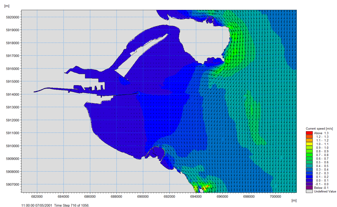
Figure 13-7 Typical spring mid flood tidal flow patterns – Post-ABR project
