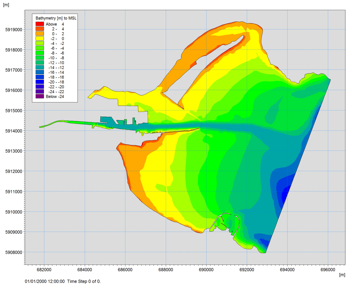
Figure 13-3 Extent and bathymetry of the 3D Dublin Port post ABR model
