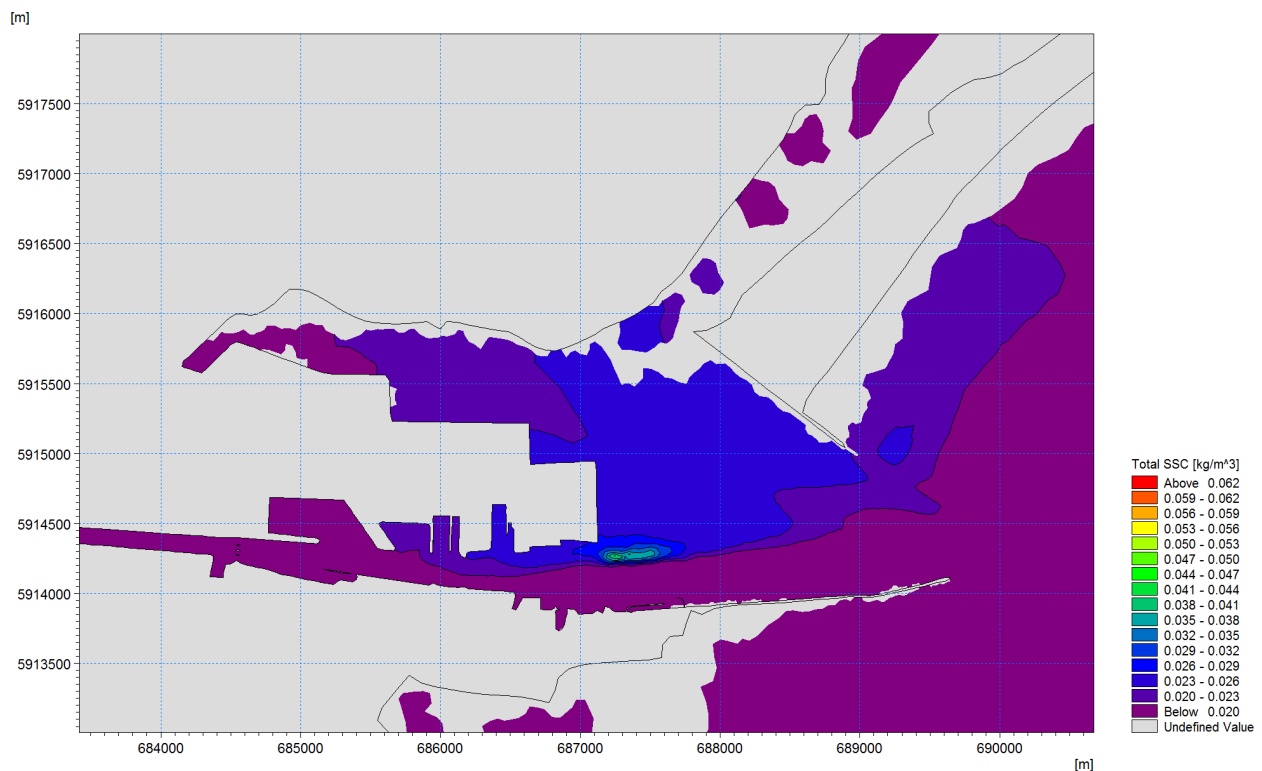
Figure 13-11 Suspended sediment concentration plume at time of low water
