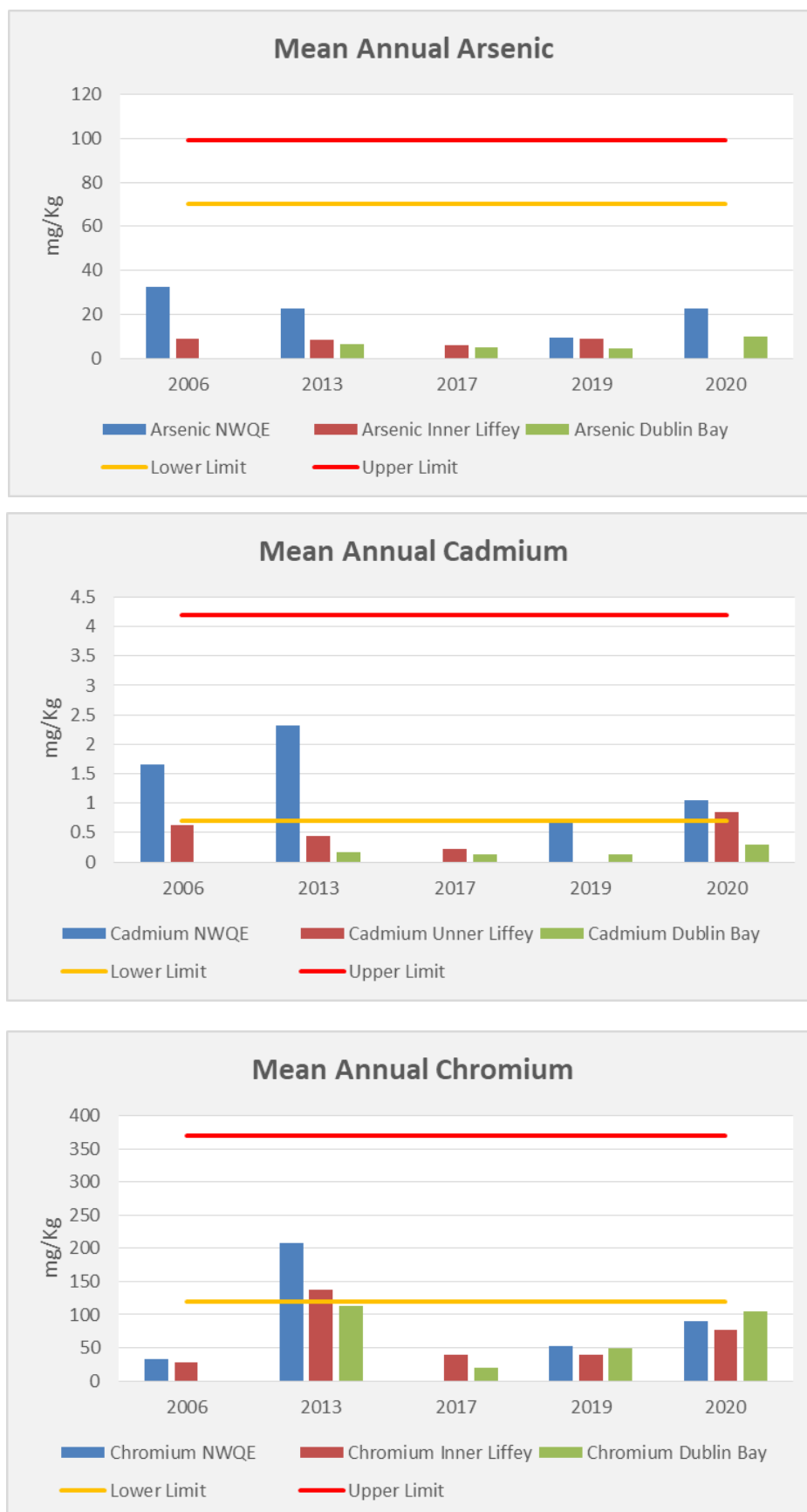
Figure 8-4 Mean Annual concentrations of metals by year and by sampling zone. Lower and upper limits where relevant are indicated by amber and red horizontal lines
