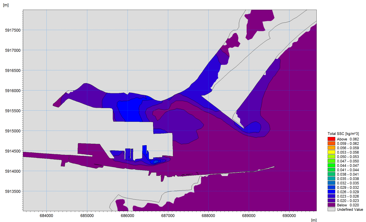
Figure 13-13 Suspended sediment concentration plume at time of high water
