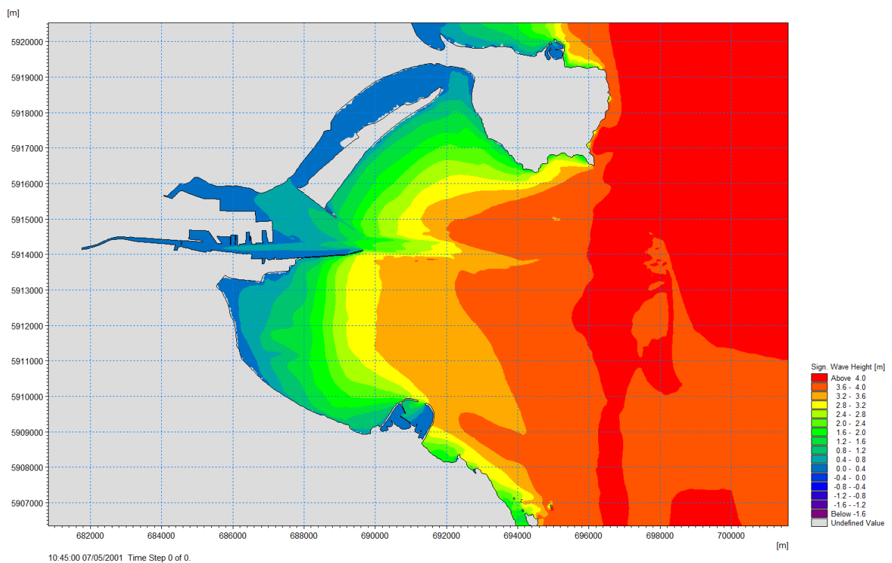
Figure 13-9 Easterly storm wave heights at spring high water – Post-ABR project
