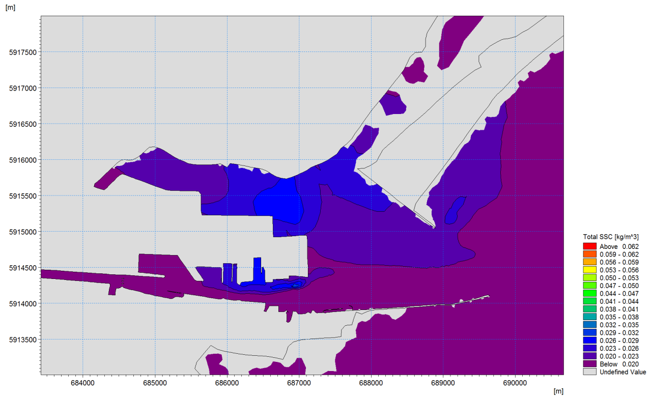
Figure 13-14 Suspended sediment concentration plume at time of mid ebb
