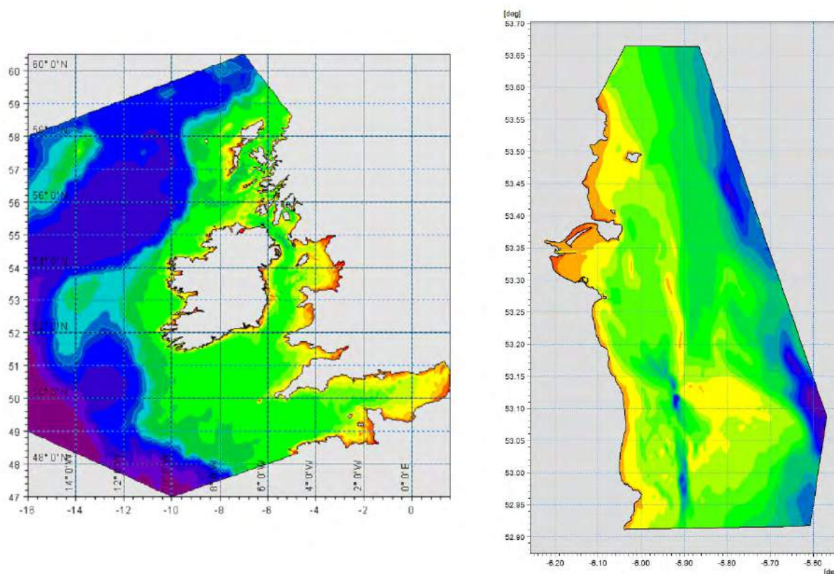
Figure 13-5 Extent and bathymetry of the ICPSS tidal surge model (left) and east coast wave model (right)
