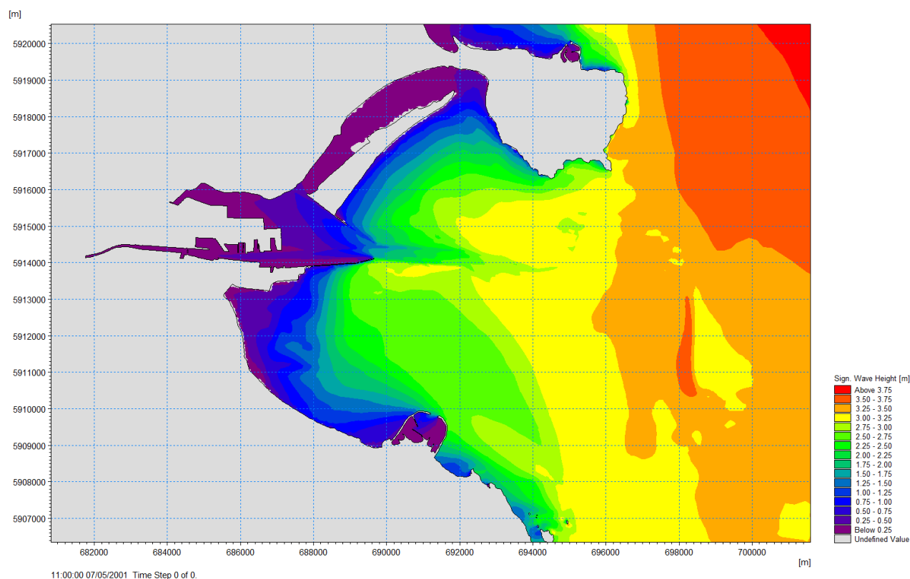
Figure 13-10 South Easterly storm wave heights at spring high water – Post-ABR project
