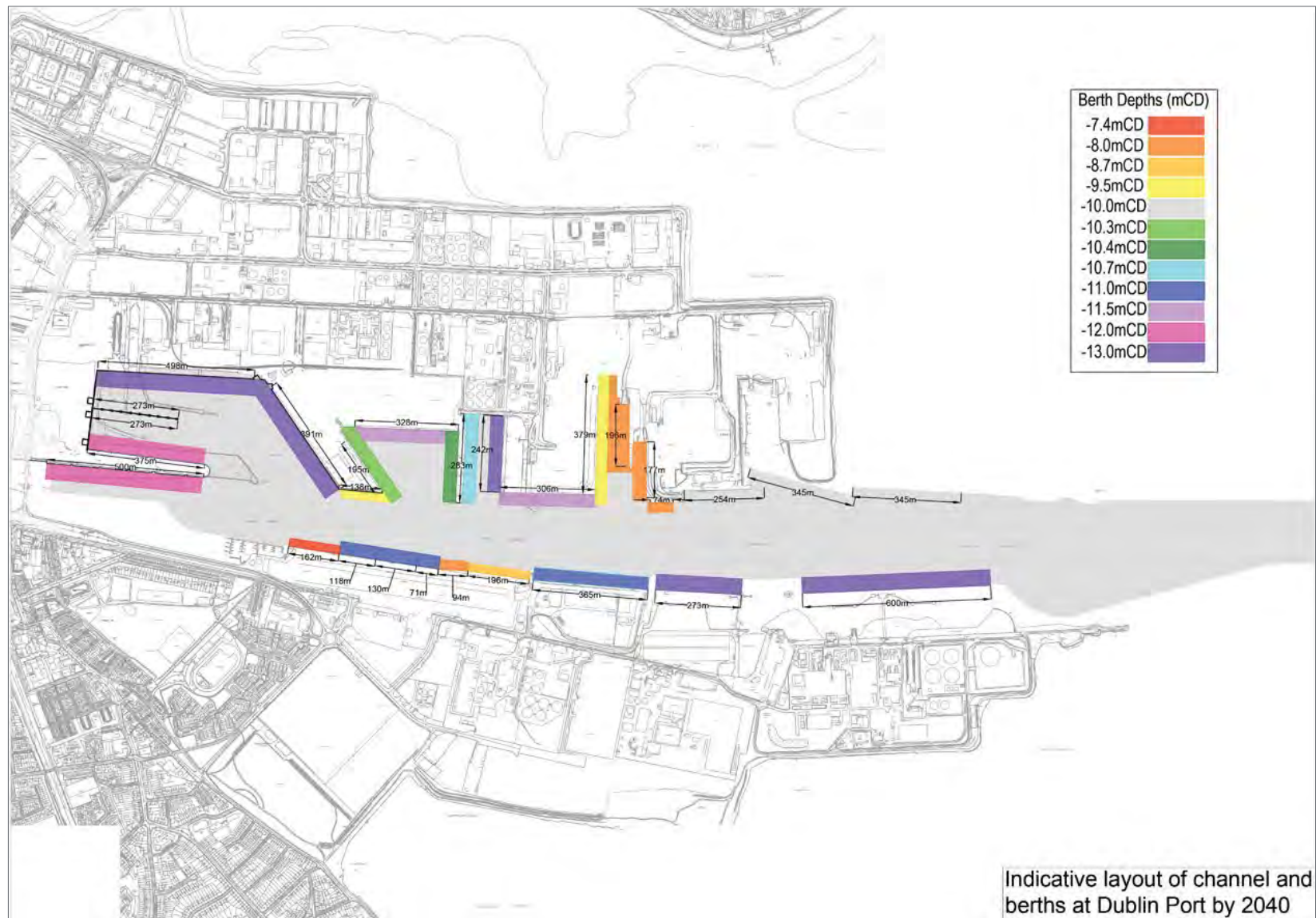
Figure 1-3 Dublin Port Masterplan 2040, reviewed 2018, Indicative Layout of channel and berths at Dublin Port at 2040
