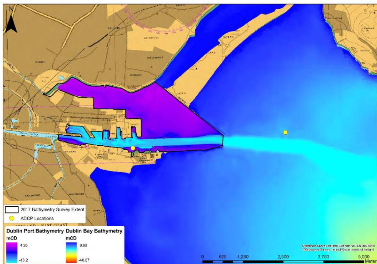
Figure 13-4 Location and coverage of the 2017 Bathymetric Survey
