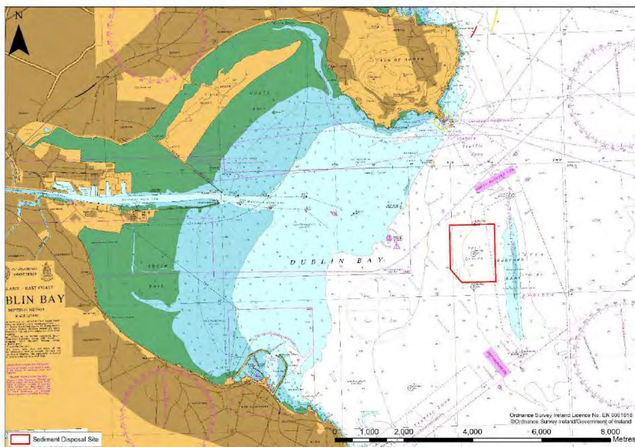
Figure 13-27 Location of the licenced dredged spoil disposal site
