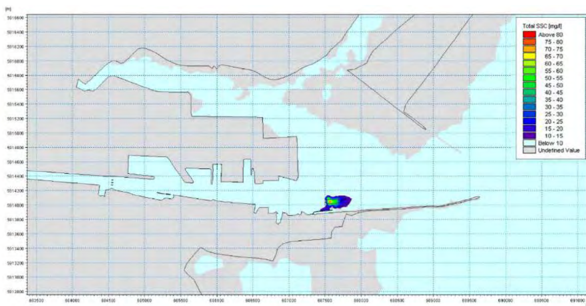
Figure 13-21 Suspended sediment concentration plume in the bottom layer during a typical low water phase of a spring tidal cycle during the capital dredging works
