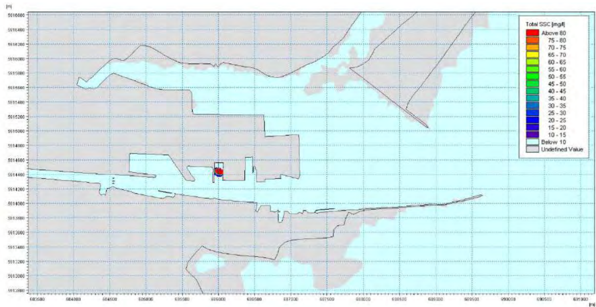
Figure 13-17 Suspended sediment concentration plume in the bottom layer during a mid flood phase of a spring tidal cycle whilst dredging within the Oil Berth
