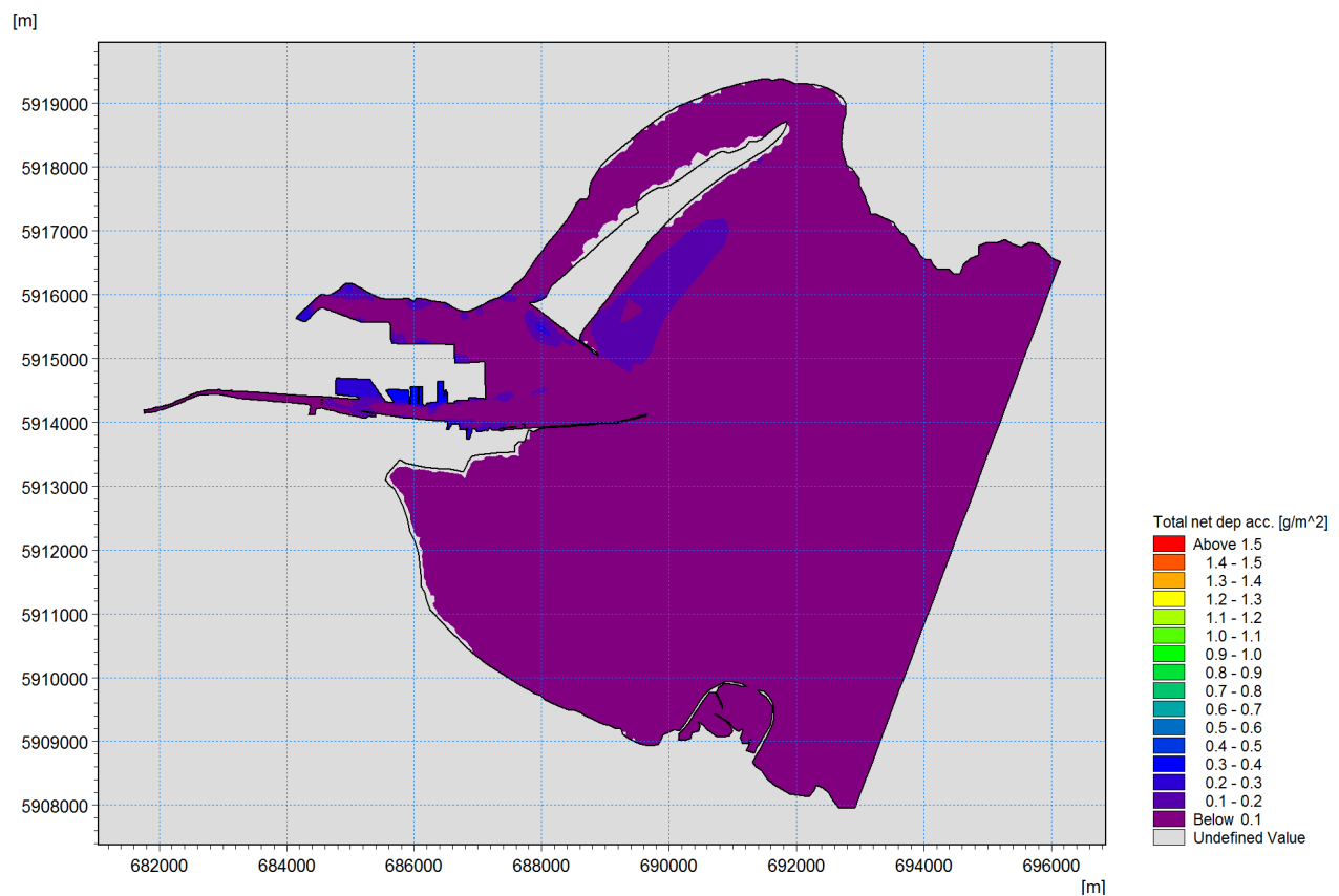
Figure 13-15 Total silt deposition after capital dredging of the middle section of the Liffey channel, Dublin Harbour
