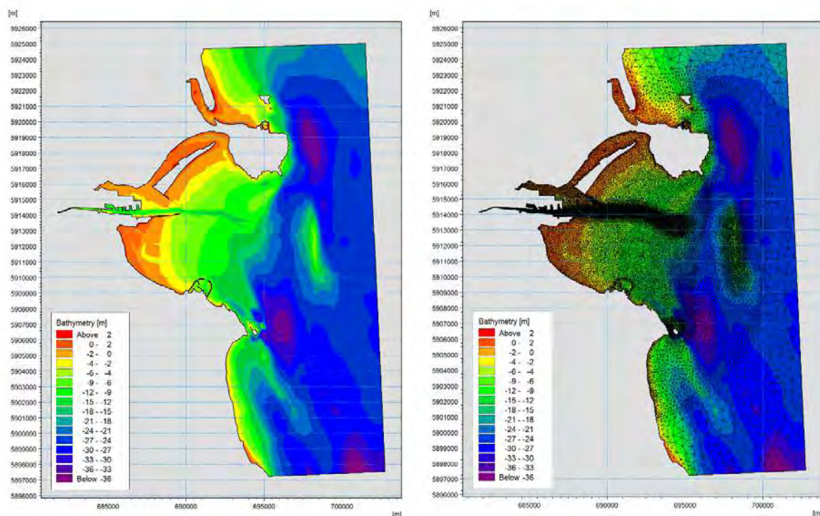
Figure 13-1 Extent and bathymetry of the Dublin Bay model (left) and the mesh structure of the Dublin Bay model (right)
