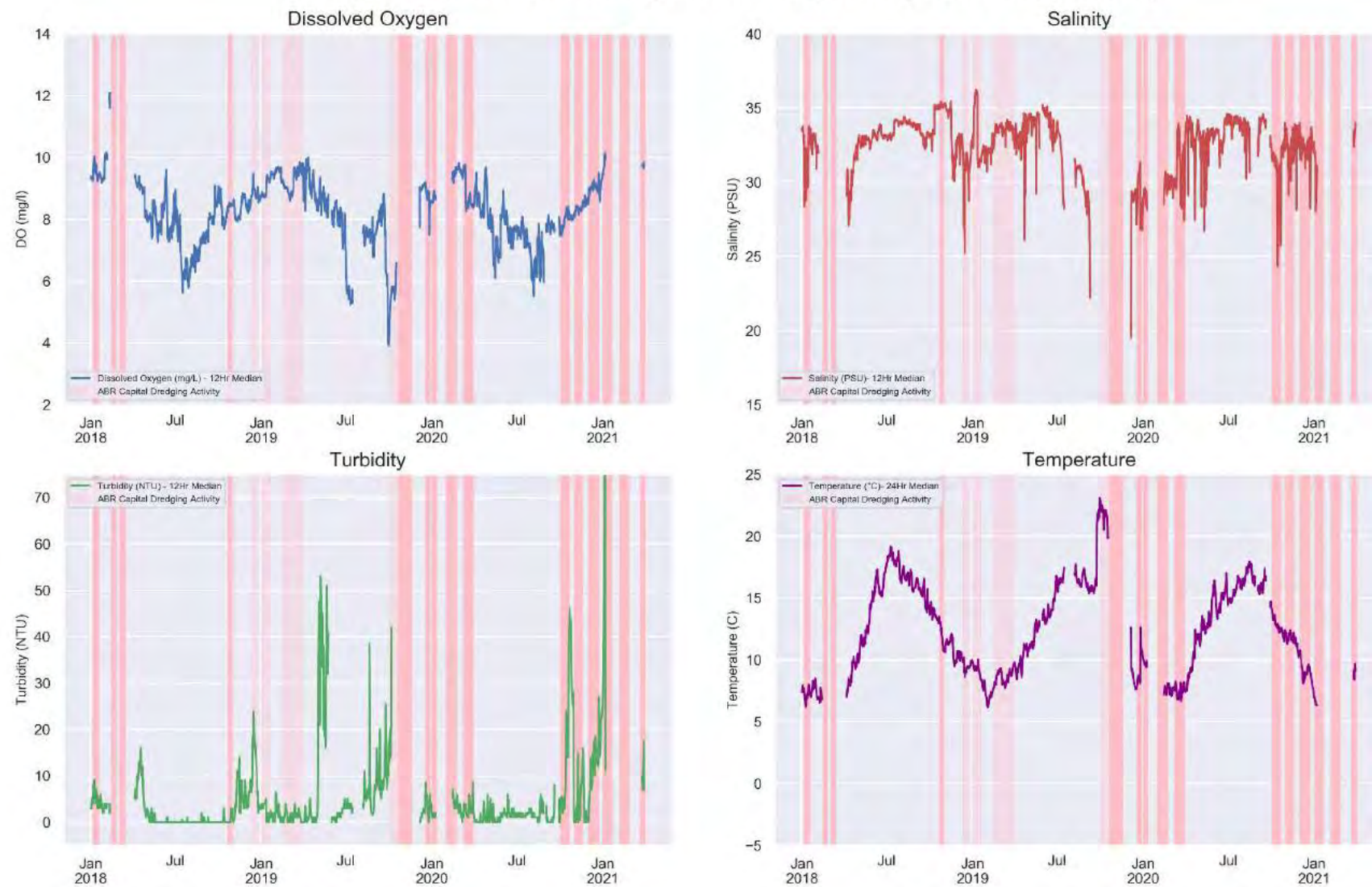
Figure 9-11 Poolbeg Monitoring Station - Water Quality Data (12 Hour Median)
