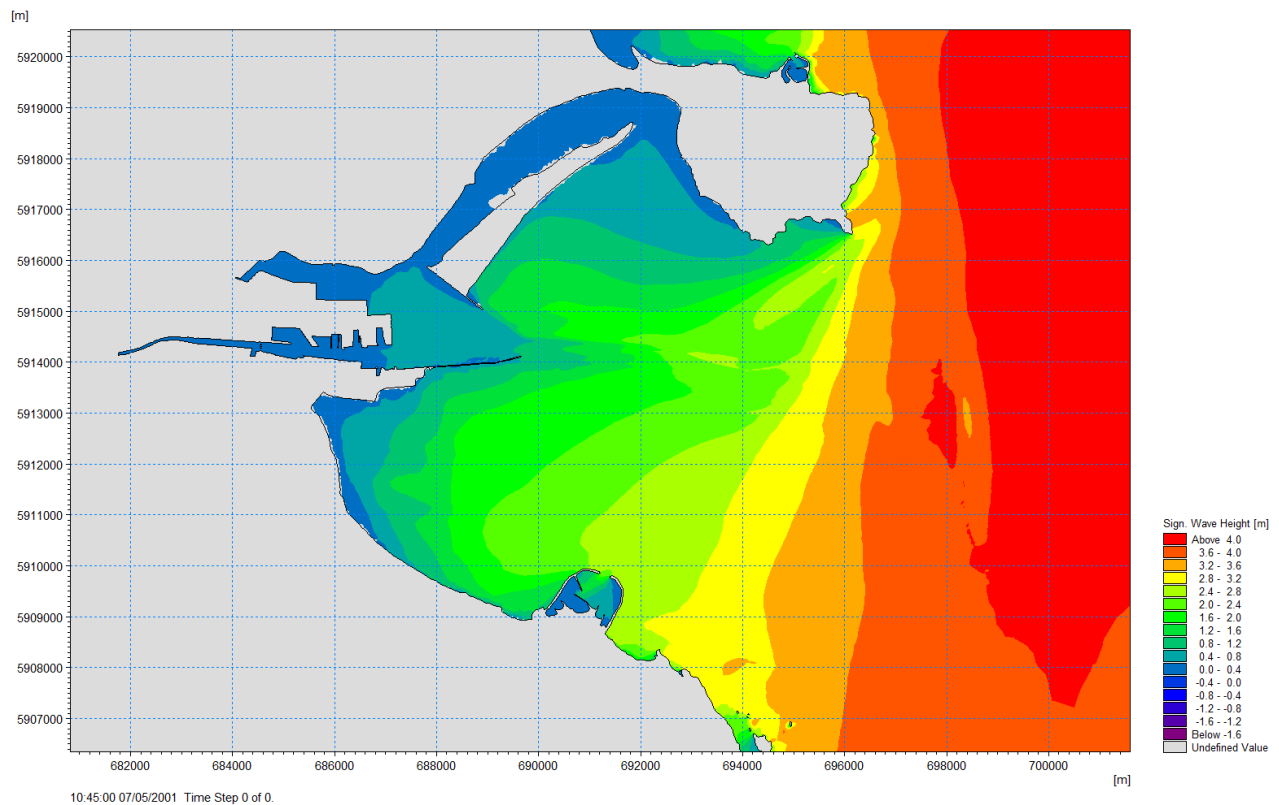
Figure 13-8 North Easterly storm wave heights at spring high water – Post-ABR project
