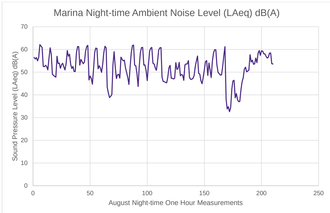
Figure 11-4 Night-time Noise Monitoring Data Recorded in August 2020 at the Marina
