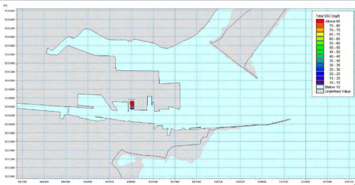
Figure 13-19 Suspended sediment concentration plume in the bottom layer during a typical mid ebb phase of a spring tidal cycle whilst dredging within the Oil Berth
