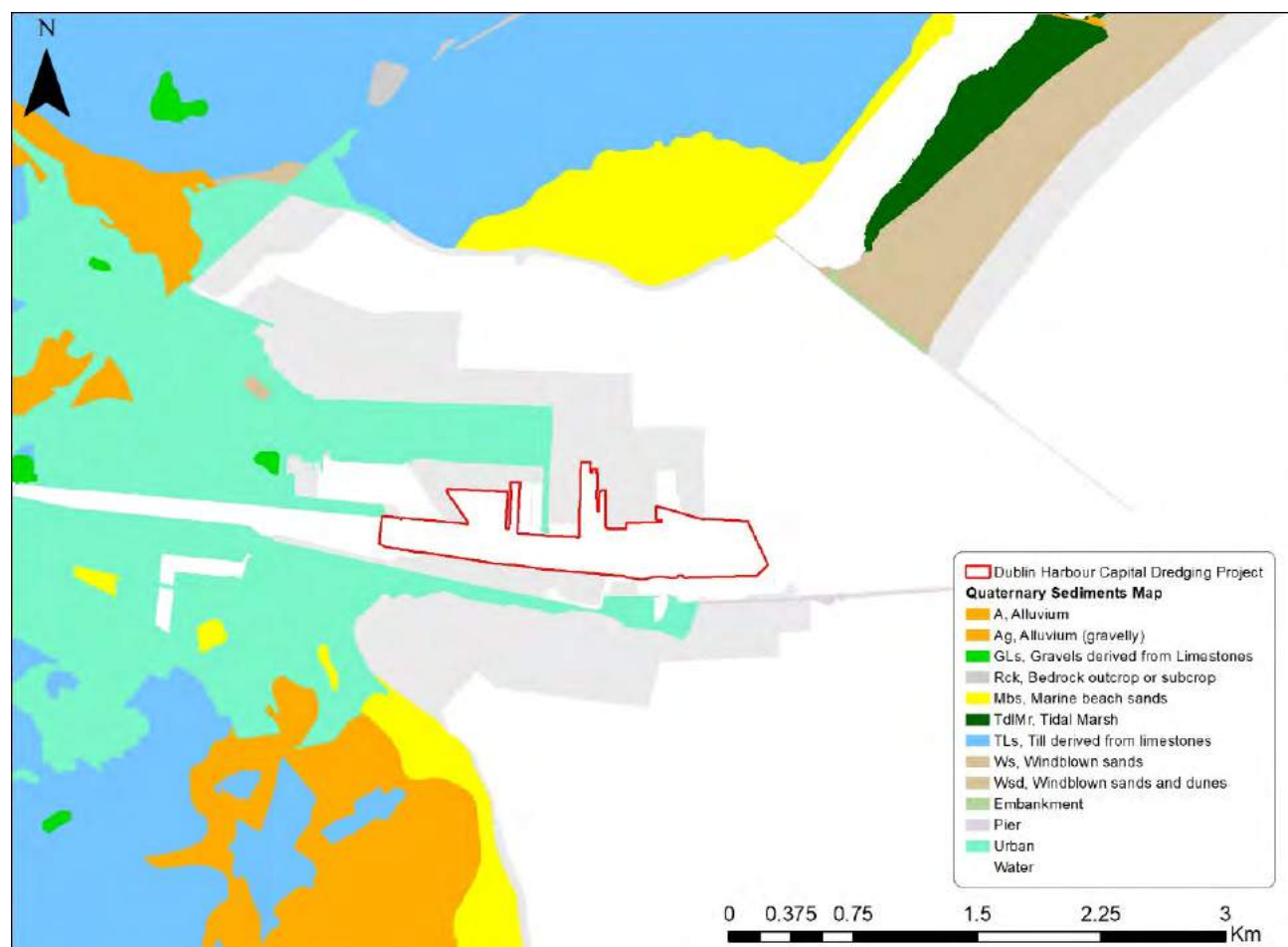
Figure 8-2 National Quaternary Geology Map of Ireland (Teagasc/GSI, 2006)
