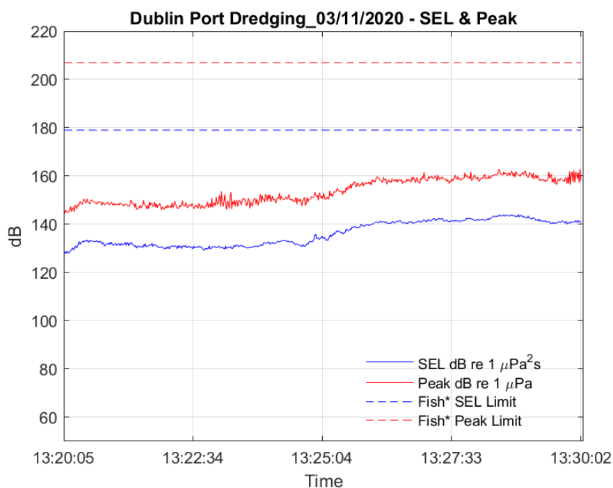
Figure 12-3 Noise levels during pass-by of TSHD Waterway
