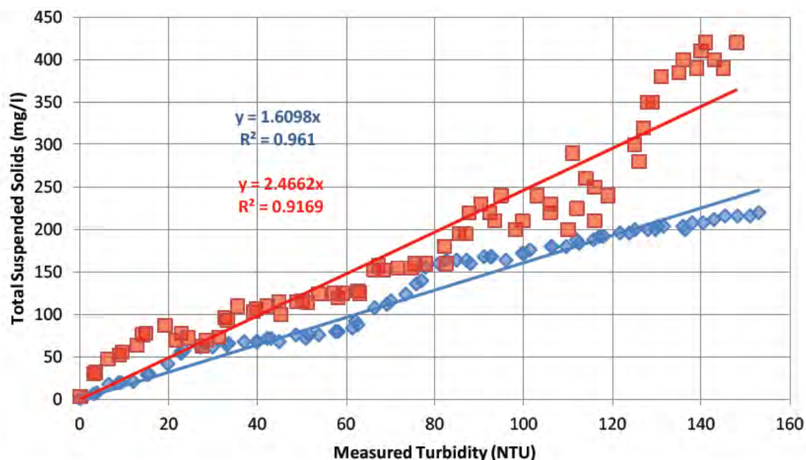
Figure 9-21: TSS versus Turbidity for suspensions of river bed silt sediment (red) and approach channel fine sand sediment (blue). Equations & r^2 values in corresponding colours for each series
