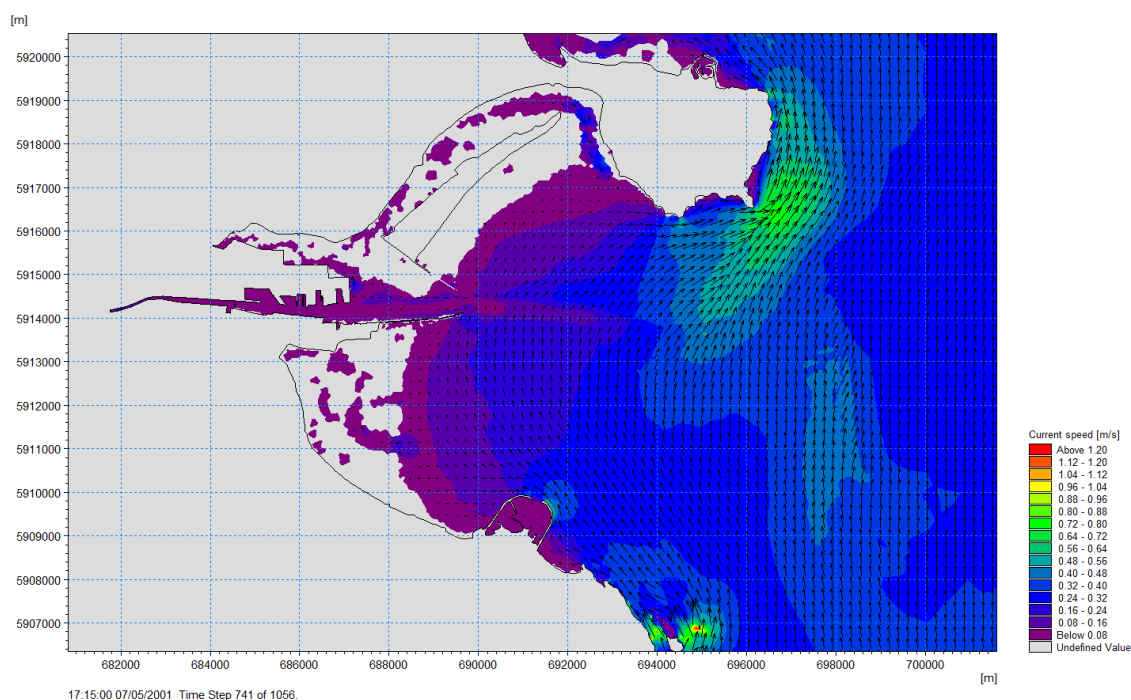
Figure 13-6 Typical spring mid ebb tidal flow patterns – Post ABR Project
