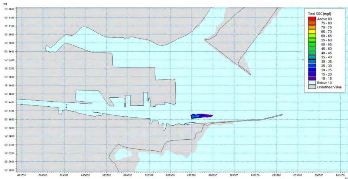
Figure 13-24 Suspended sediment concentration plume in the bottom layer during a typical mid ebb phase of a spring tidal cycle during the capital dredging works
