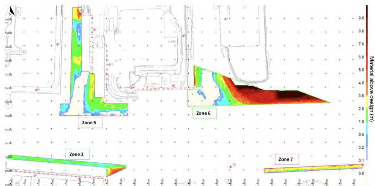
Figure 3-3 Plot showing depth of material between current bed level and design depth (metres) – Zone 2,5,6 and 7
