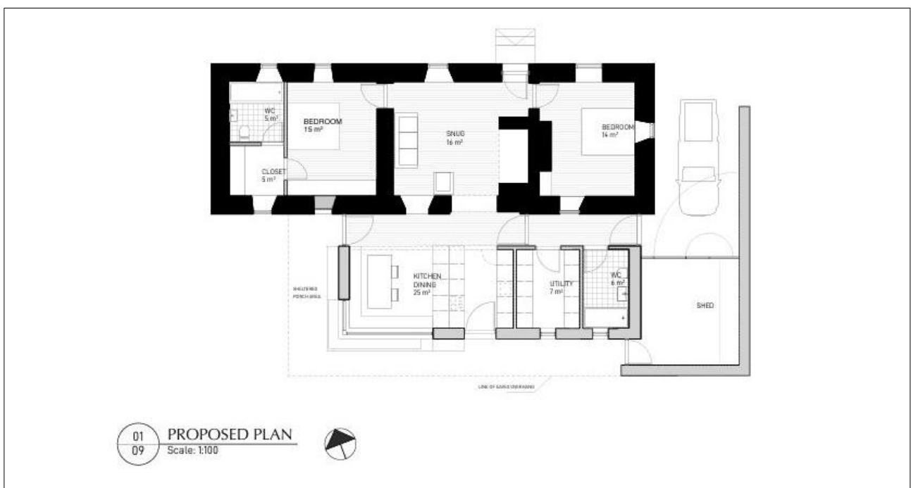
Figure 1b: Proposed layout of Gamekeeper's Lodge with original footprint of Lodge shown in black and new sections shown in grey.
