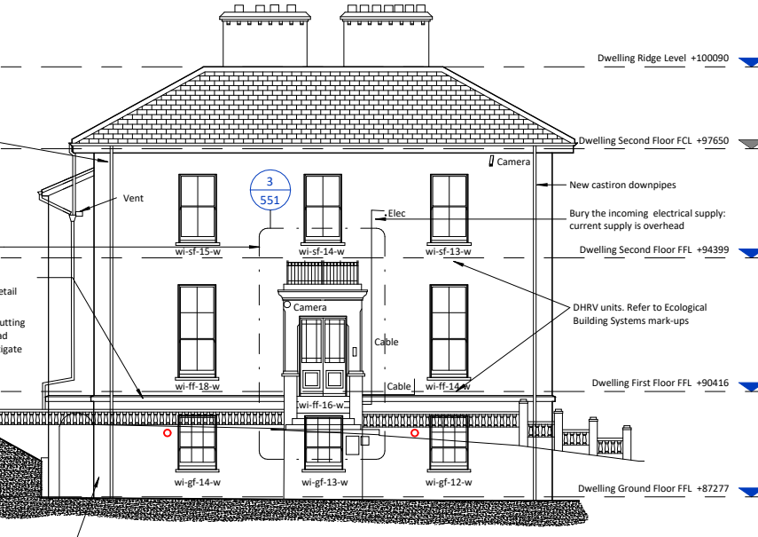
5 Dwelling Proposed West Elevation 1:100
