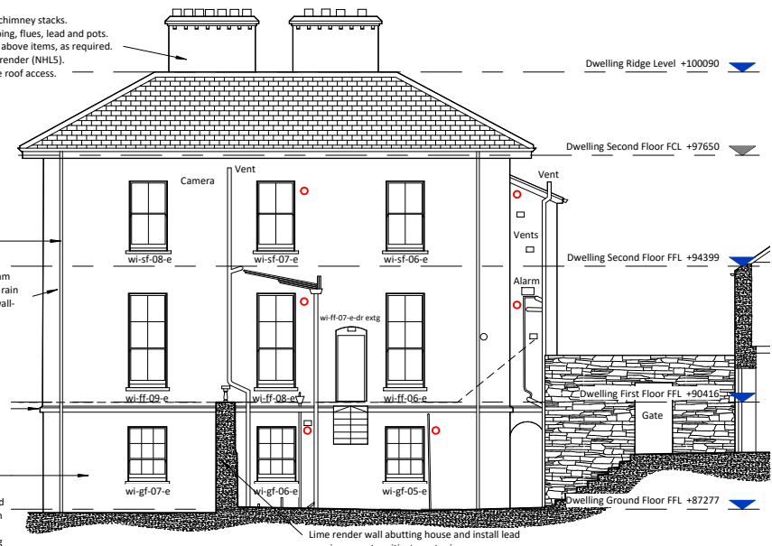
8 Dwelling Proposed East Elevation 1:100
