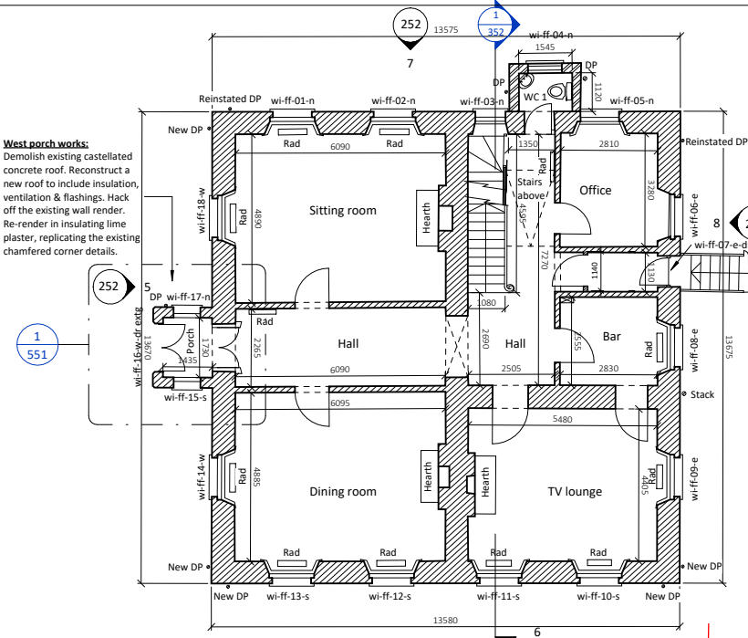
6 Dwelling Proposed First Floor Plan
