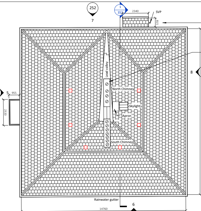
8 Dwelling Proposed Roof Plan
