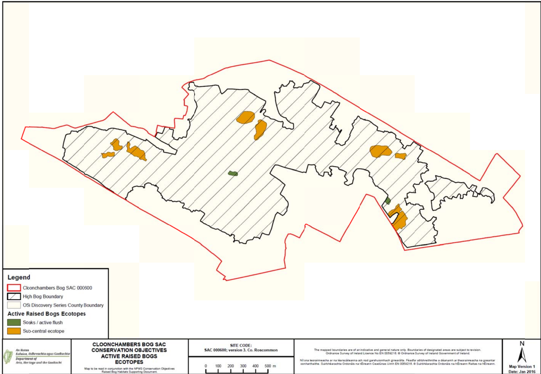
Map 2: Distribution of raised bog ecotopes on Cloonchambers Bog.
