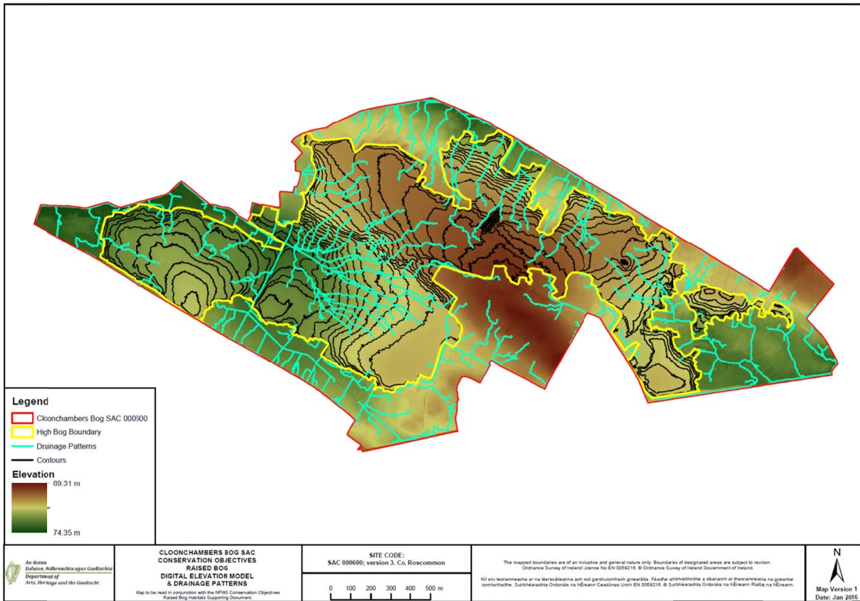
Map 3: Digital elevation model and drainage patterns at Cloonchambers Bog.
