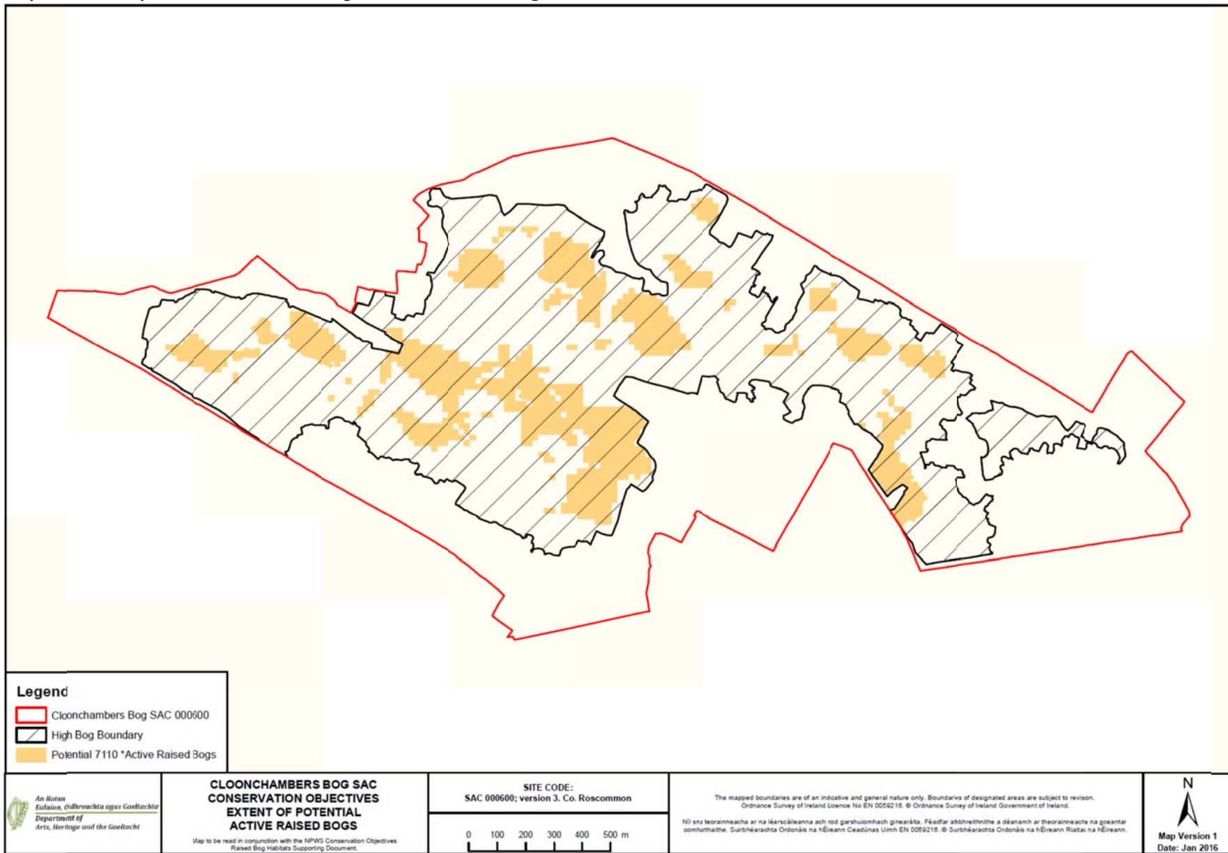
Map 1: Extent of potential active raised bog on Cloonchambers Bog.
